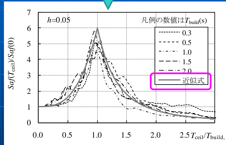
(b) S_{af}(T_{ceil})/S_{af}(0) - T_{ceil}/T_{build} 関係
